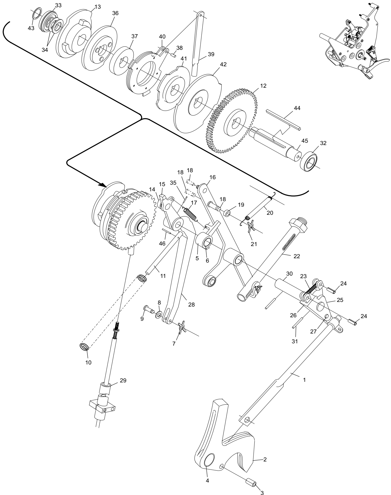
Detector Main Shaft Assembly
