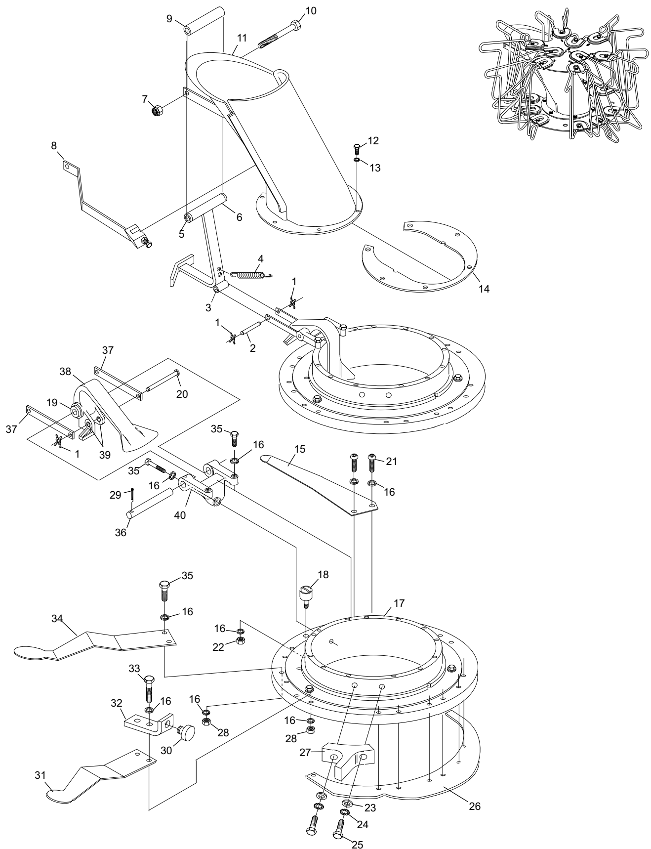
Turret Ring and Index Assembly
